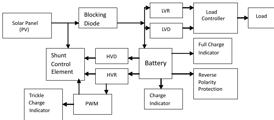
Figure 1. Block diagram of a battery charge-controller
